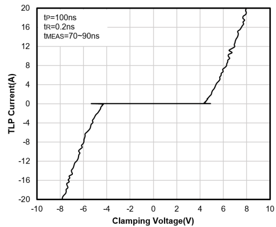
TLP Curve
